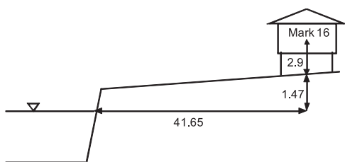
Figure 3.4.10.3 Section view around Mark 16
