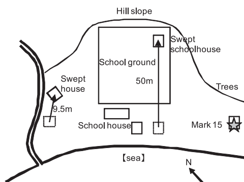
Figure 3.4.11.2 Location of measured tsunami trace, mark 15, in Reona
