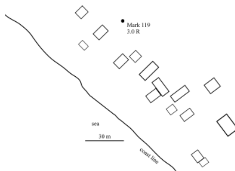
Figure 3.2.5.1 Trace height surveyed in Mengge
