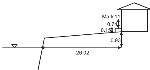
Figure 3.1.6.2 Topographic transect near Mark 11
