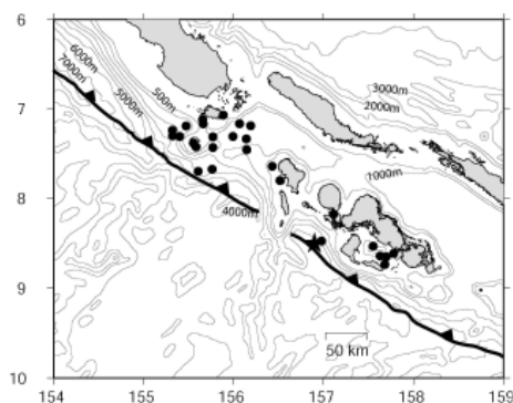
Fig. 2.2 Aftershock distribution of the 2007 Solomon event. A star is the epicenter of the main shock. Circles are one-day aftershocks.
