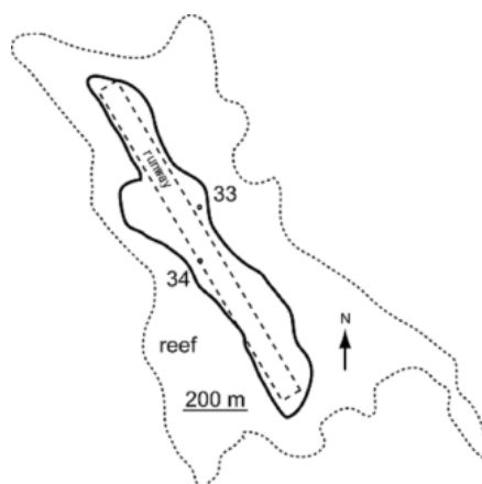
Fig. 3.1.8.1 Coastal line (solid line) and reef edges (dotted line) around Gizo airport
