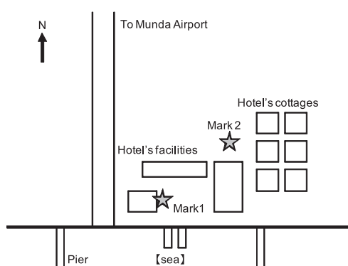
Figure 3.5.3.3 Locations of measured tsunami traces, Marks 1 and 2, in Munda
