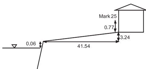
Figure 3.1.4.4 Transect near Mark 25
