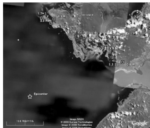
Figure 3.5.3.1 Measurement points in Munda and epicenter
