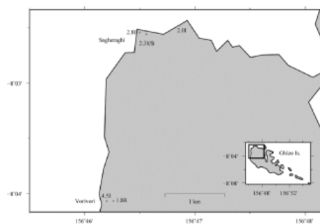
Figure 3.1.1.4 Survey locations and tsunami trace heights at Sagheraghi and Vorivori
