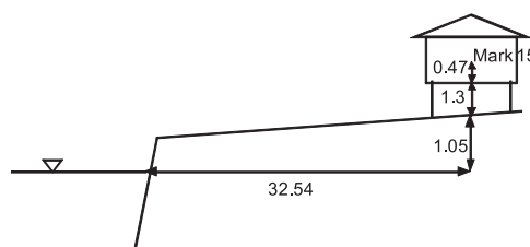
Figure 3.4.11.3 Transect near Mark 15
