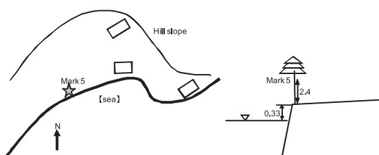
Figure 3.2.4.2 Horizontal and section views around Mark 5
