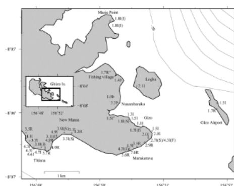
Figure 3.1.1.3 Survey locations and tsunami trace heights from Titiana through Gizo to Marie Point
