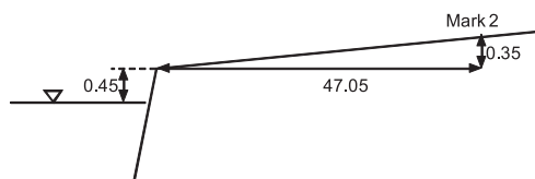
Figure 3.5.3.5 Transect near Mark 2
