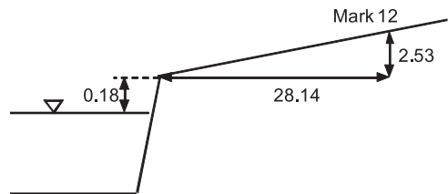
Figure 3.4.12.2 Section view around Mark 12
