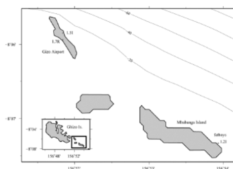
Figure 3.1.1.5 Survey locations and tsunami trace heights at Gizo Airport and fatboys
