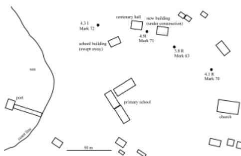
Figure 3.2.6.1 Trace heights surveyed in Lengana
