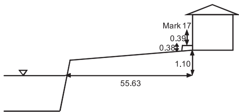
Figure 3.4.10.4 Section view around Mark 17
