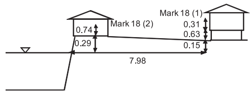
Figure 3.4.3.3 Transect near Marks 18 (1) and 18 (2)
