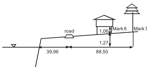
Figure 3.1.12.3 Topographic transect near Marks 6 and 7
