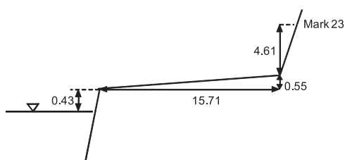
Figure 3.1.4.2 Transect near Mark 23
