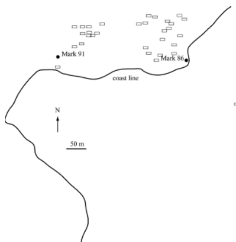
Figure 3.4.5.1 Tsunami survey points at Niarovai, Vella Lavella Island.
