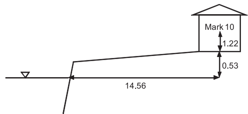
Figure 3.1.6.3 Topographic transect near Mark 10
