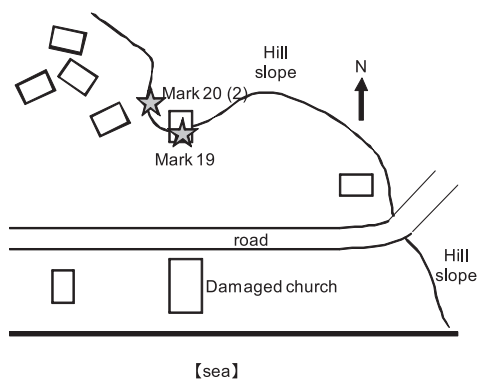
Figure 3.1.2.2 Locations of measured tsunami traces, Marks 19 and 20 (2), in Titiana
