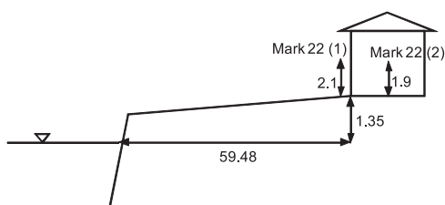
Figure 3.1.3.3 Topographic transect near Marks 22 (1) and 22 (2)
