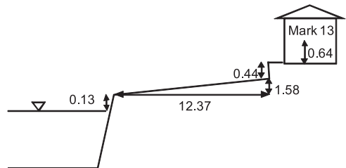
Figure 3.4.12.3 Section view around Mark 13
