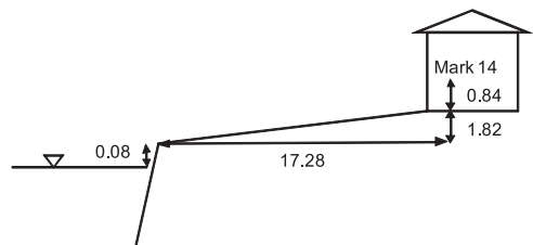
Figure 3.4.12.4 Section view around Mark 14
