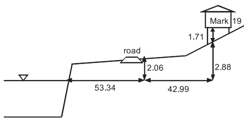
Figure 3.1.2.3 Topographic transect near Mark 19
