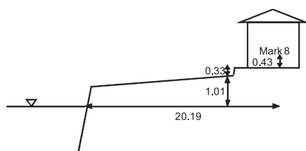
Figure 3.1.11.3 Topographic transect near Mark 8
