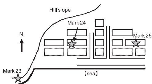
Figure 3.1.4.1 Locations of measured tsunami traces, Marks 23, 24 and 25, in Marakerava 3
