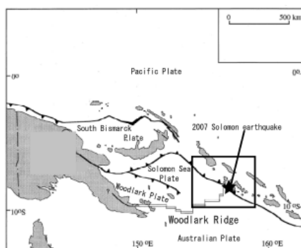
Fig. 2.1 Plate boundaries around the source region of the earthquakes. (from Tregoning et al., 1998) A star shows the epicenter of the 2007 Solomon earthquake. A rectangular shows the area of Fig. 2.2.
