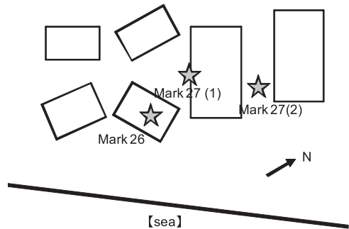
Figure 3.1.5.1 Locations of measured tsunami traces, Mark 26, 27 (1) and 2 (2) in Marakerava 1
