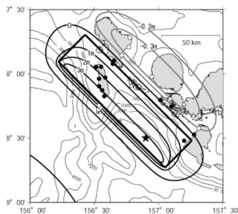
Fig. 2.8. The vertical deformation pattern using a fault model with a depth of the shallowest edge of the fault model of 5 km. The rests of the faults parameters are same as the estimated fault model.
