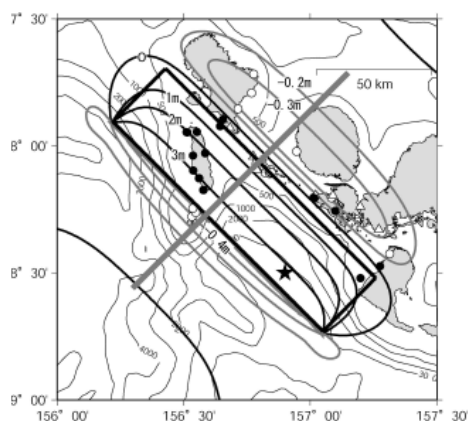
Fig. 2.6 The fault model of the 2007 Solomon earthquake. Solid contours show the uplift (m), with an interval of 1m, and shaded contours show the subsidence (m), with an interval of 0.1 m. An shaded line is the cross-section line for Fig. 2.7. Black dots shows the places where coseismic uplifts were observed. Triangles show the places where no coseismic deformation were observed. Open dots shows the places where coseismic subsidences were observed.
