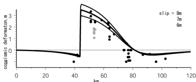
Fig. 2.7. Cross-section of the vertical deformation along the shaded line in Fig. 2.6. Dots show the observed coseismic deformation data. Shaded dots are the coseismic uplifts measured from the top of the coral heads which may be less than the actual uplifts.
