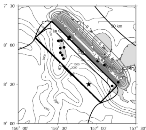
Fig. 2.9 The vertical deformation pattern using a fault model with a dip angle of 15 degree. The rests of the faults parameters are same as the estimated fault model.
