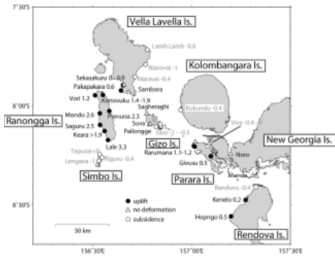
Fig. 2.3 Coseismic vertical deformation by the 2007 Solomon earthquake
