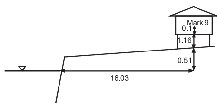
Figure 3.1.11.4 Topographic transect near Mark 9
