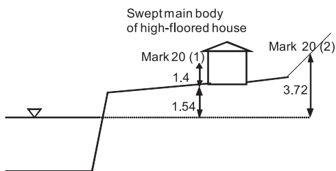
Figure 3.1.2.4 Topographic transect near Mark 20 (2)
