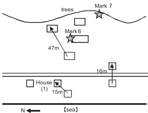
Figure 3.1.12.2 Location of measured tsunami traces, Marks 6 and 7, in Sagheraghi
