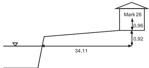
Figure 3.1.5.2 Transect near Mark 26
