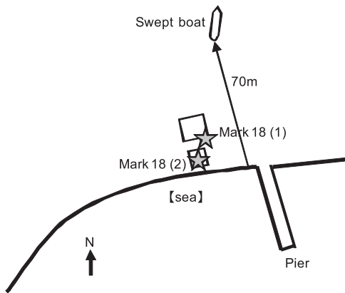
Figure 3.4.3.2 Locations of measured tsunami traces, Marks 18(1) and 18 (2), in Vonunu
