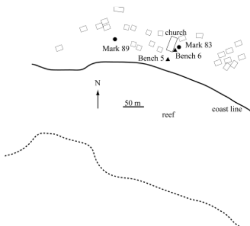
Figure 3.4.2.1 Location map of tsunami survey points and benchmarks at Sambora
