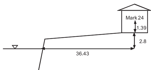
Figure 3.1.4.3 Transect near Mark 24
