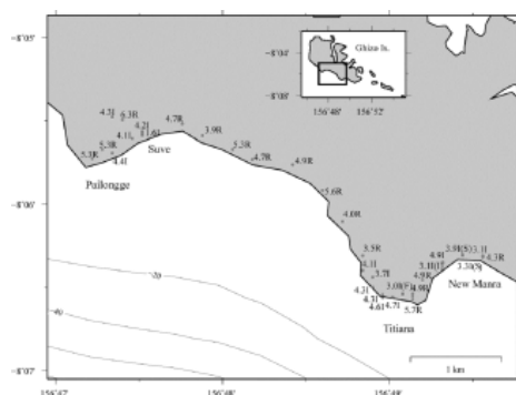
Figure 3.1.1.2 Survey locations and tsunami trace heights from Pailonge through Titiana to New Manra
